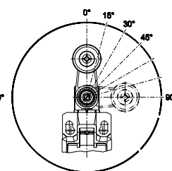
Adjustable lever
